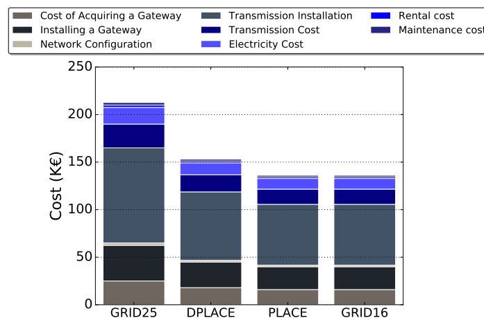
Figure 8. Total cost per specific service for analyzed LoRaWAN gateway placement models.
