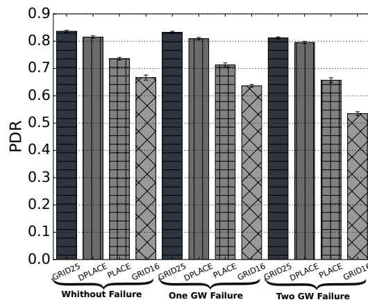
Figure 3. Packet Delivery Ratio (PDR) for analyzed LoRaWAN gateway placement models.
