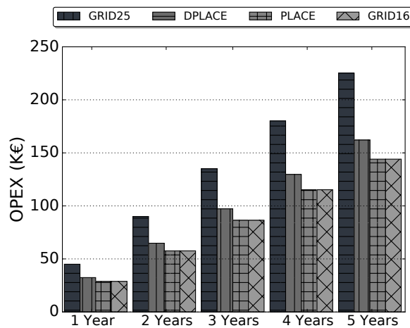
Figure 7. OPEX for analyzed LoRaWAN gateway placement models.
