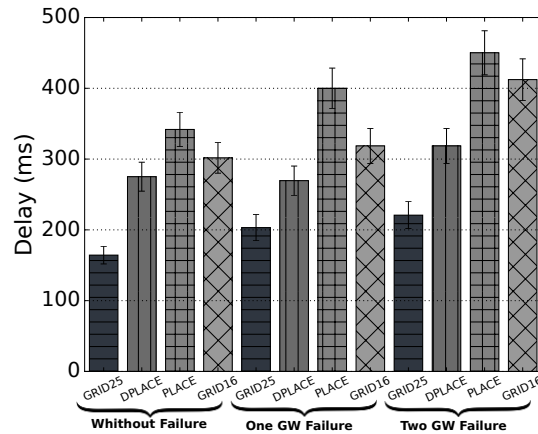
Figure 5. Mean delay for analyzed LoRaWAN gateway placement models.
