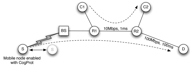
Fig. 4. Simulated topology.
