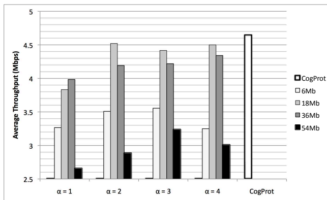
Fig. 7. Average TCP throughput with changing conditions.
